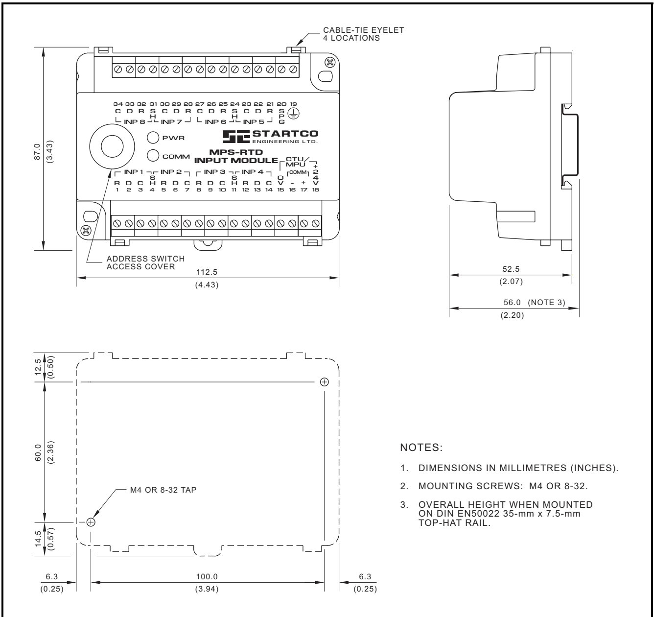
FIGURE 2.4 MPS-RTD Outline and Mounting Details.
