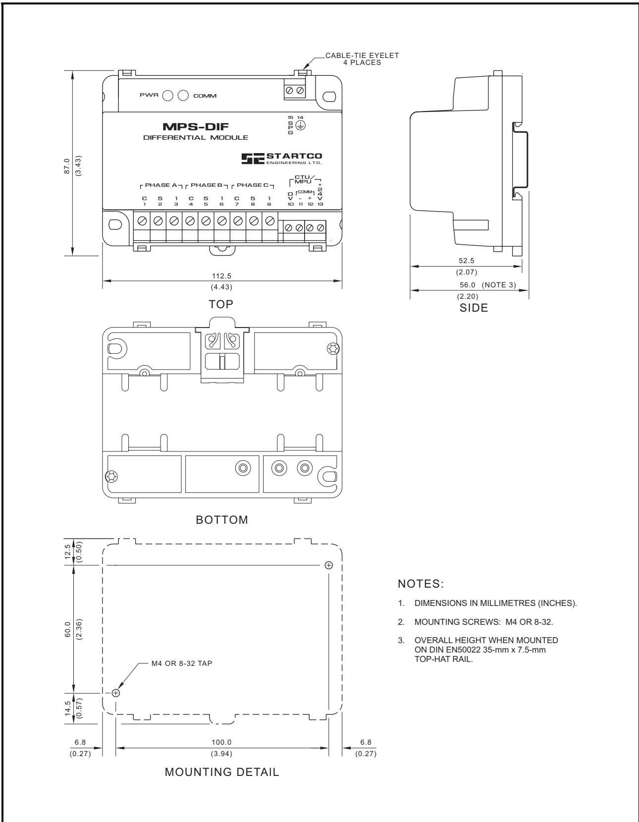
FIGURE 2.5 MPS-DIF Outline and Mounting Details.
